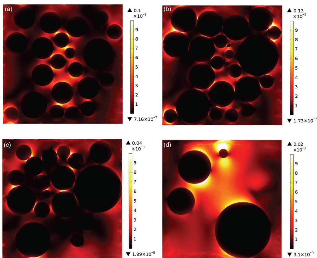
Fig. 9 Time-averaged Poynting vector ( W/m^2 ) on the glass substrate and the air medium of the nanoparticles under \lambda = 532 nm, TE (Y-pol.) polarized light at different distances ( z ) above the glass substrate for standard deviation 84-nm nanoparticle packings: (a) z = 50 nm, (b) z = 100 nm, (c) z = 200 nm, and (d) z = 400 nm.
