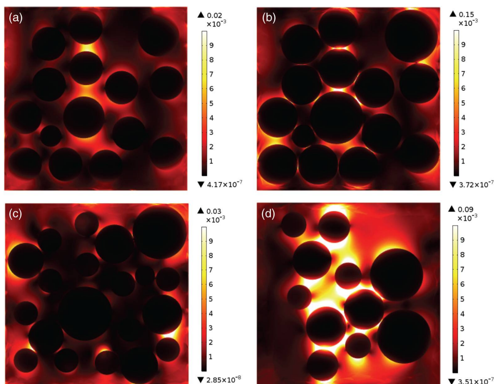
Fig. 7 Time-averaged Poynting vector ( W/m^2 ) on the glass substrate and the air medium of the nanoparticles under \lambda = 532 nm, TE (Y-pol.) polarized light at different distances ( z ) above the glass substrate for standard deviation 12-nm nanoparticle packings: (a) z = 50 nm, (b) z = 100 nm, (c) z = 200 nm, and (d) z = 400 nm.
