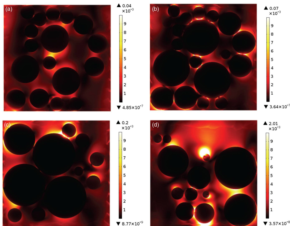
Fig. 8 Time-averaged Poynting vector ( W/m^2 ) on the glass substrate and the air medium of the nanoparticles under \lambda = 532 nm, TE (Y-pol.) polarized light at different distances ( z ) above the glass substrate for standard deviation 48-nm nanoparticle packings: (a) z = 50 nm, (b) z = 100 nm, (c) z = 200 nm, and (d) z = 400 nm.
