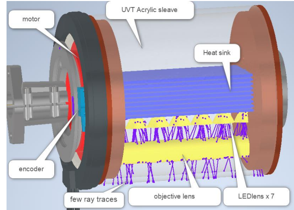
FIGURE 5. Model of acrylic pacer of lithography module with ray traces.
