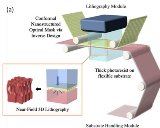
FIGURE 1. Diagram of proposed 3D holographic pattern manufacturing system.
