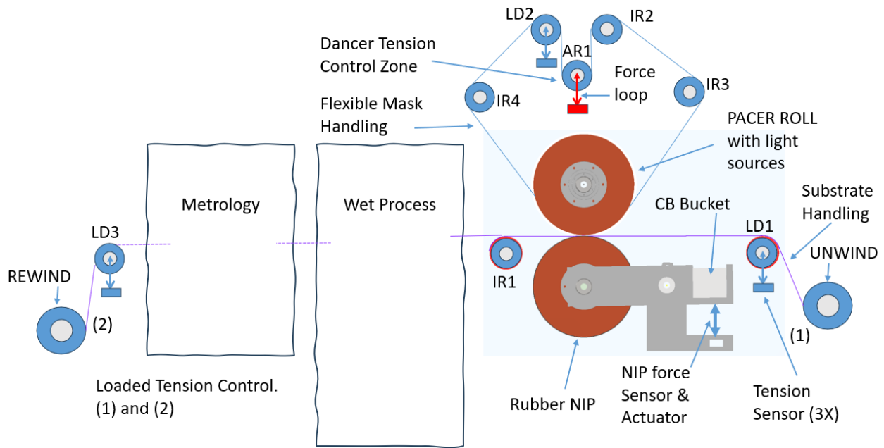
FIGURE 2. Diagram of Planned Manufacturing System.
