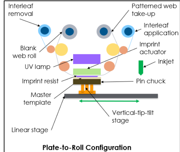
FIGURE 4. Nanoimprint mask-production system [6].
