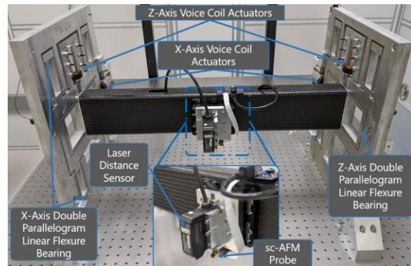
FIGURE 3. Pictured is the nanopositioning AFM metrology system, part of the proposed system's metrology module.
