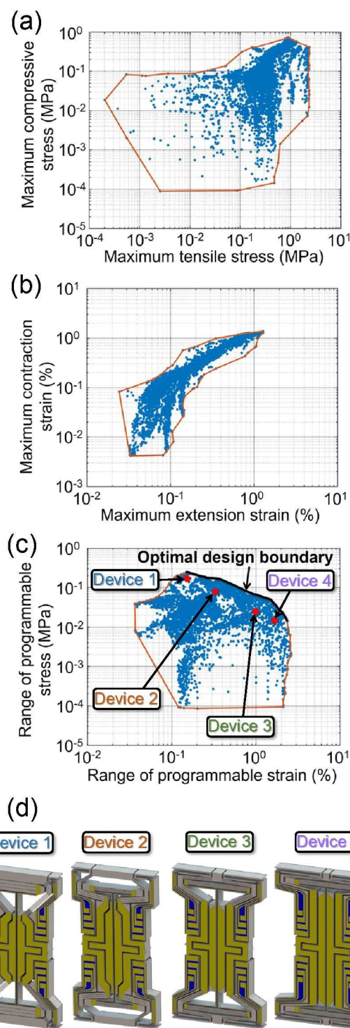
Figure 2. Performance boundary plots generated from a parameter sweep of the design of Fig. 1 showing (a) maximum compressive and tensile stresses, (b) maximum contraction and extension strains, and (c) the ranges of programmable stress and strain for each design version considered in the sweep; (d) four design versions (i.e., devices) that are close to and parallel the optimal design boundary.
